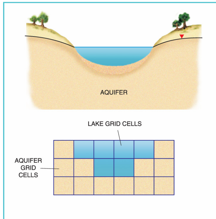
Figure 1. Cell discretization used by the Lake package (taken from Merritt, L.M. and Konikow, L.F., 2000, Documentation of a computer program to simulate lake-aquifer interaction using the MODFLOW ground-water flow model and the MOC3D solute-transport model: U.S. Geological Survey Water-Resources Investigations Report 00-4167 ).
